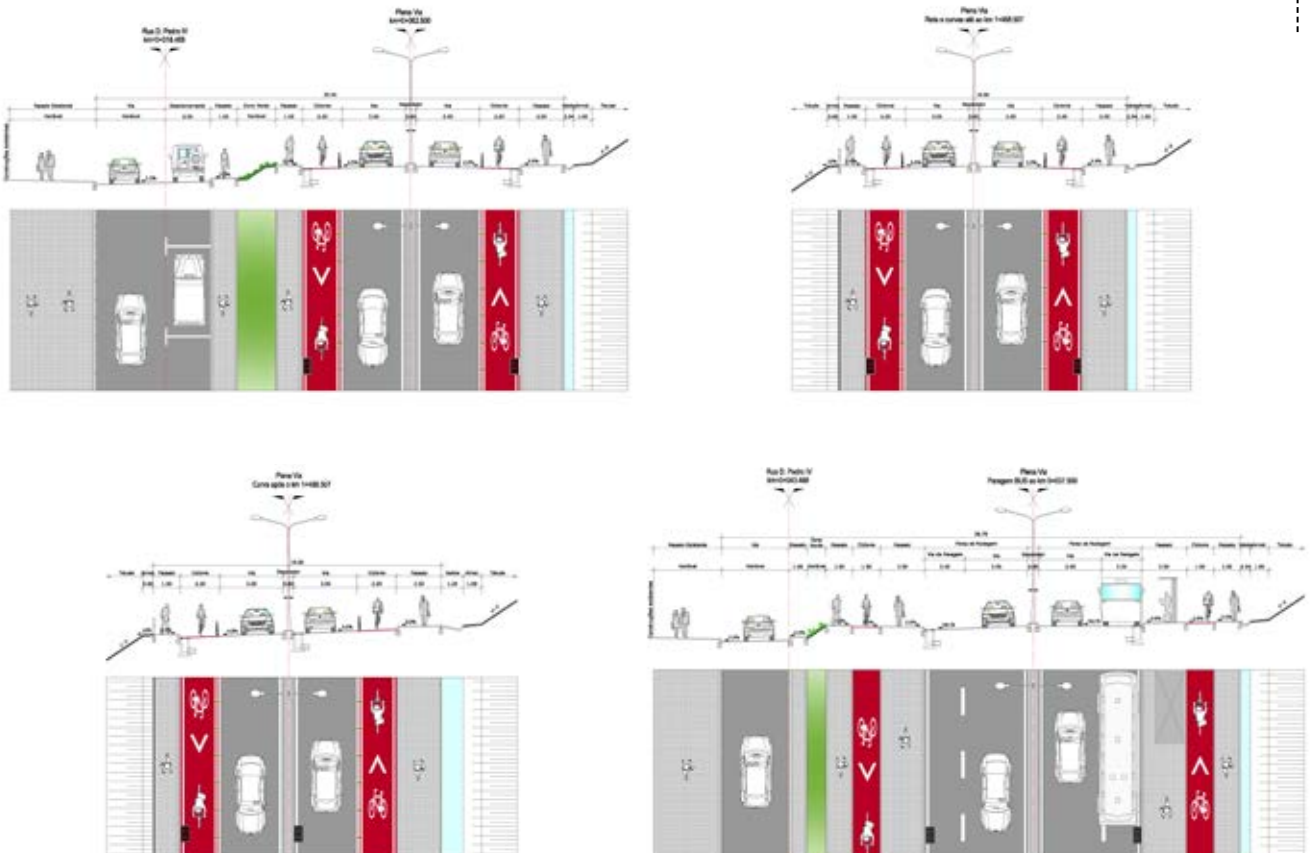
CROSS-SECTIONS
