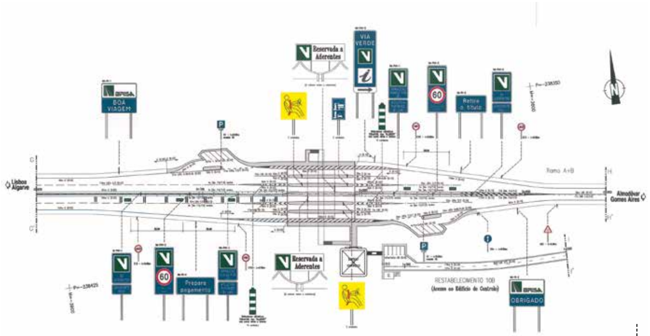
TOLL BOOTH AREA TRAFFIC SIGNS
